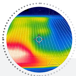
Thermal image of oil cooler
